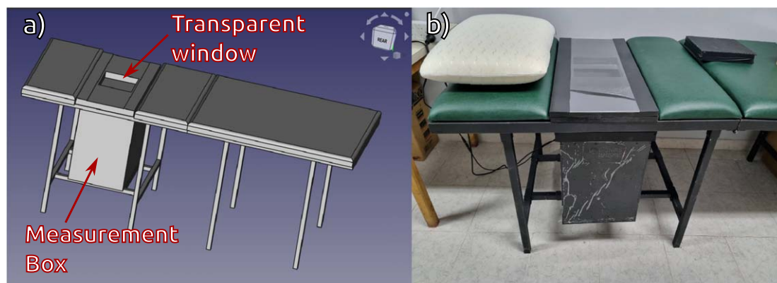
Figure 5. 3D rendering of the stretcher with the measurement box installed (a) and a photo of the actual device (b). The measurement box is removable for transport and maintenance.
